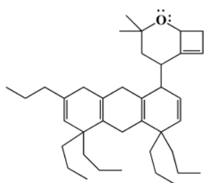
3,3-dimethyl-5-(4,4,5,5,7-pentapropyl-1,4,5,8,9,10-hexahydroanthracen-1-yl)-2-oxabicyclo[4.2.0]oct-6-ene
