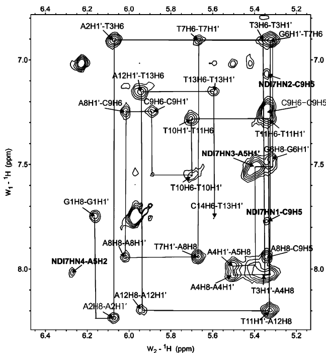
Figure 7. Expansion of the NOESY spectrum (mixing time 60 ms, pH 7.5, 27 ^\circ\text{C} ) of the 3 –( 4 ) 2 complex. Sequential aromatics to \text{H}1' connectivities are shown as lines.
